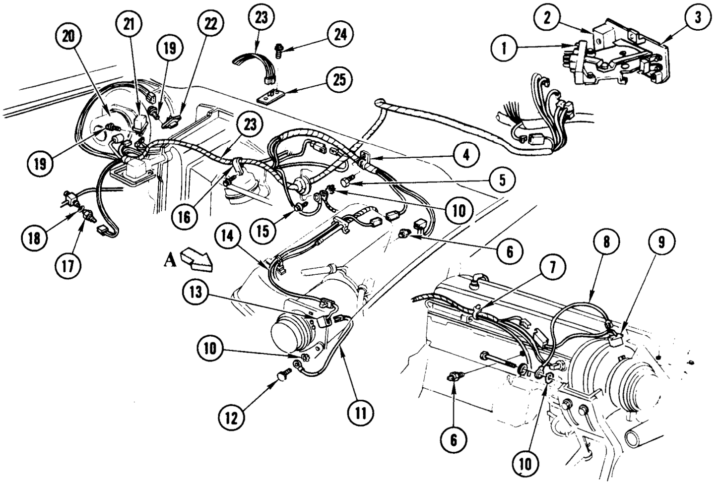
VIEW A - FOR 6 CYL
